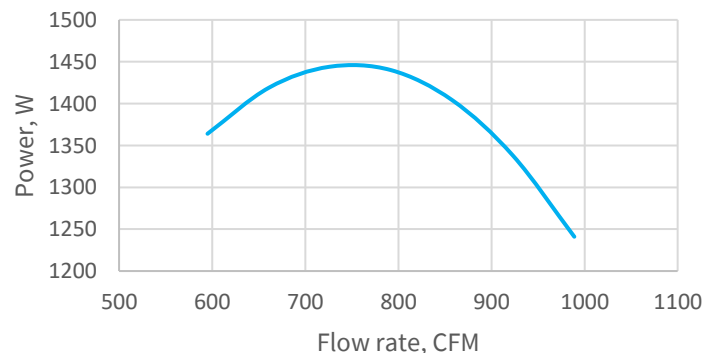
Galeforce 135 Power Curve
