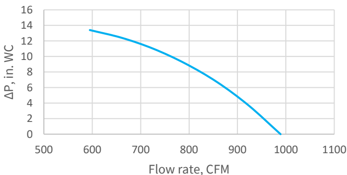
Galeforce 135 Performance Curve
