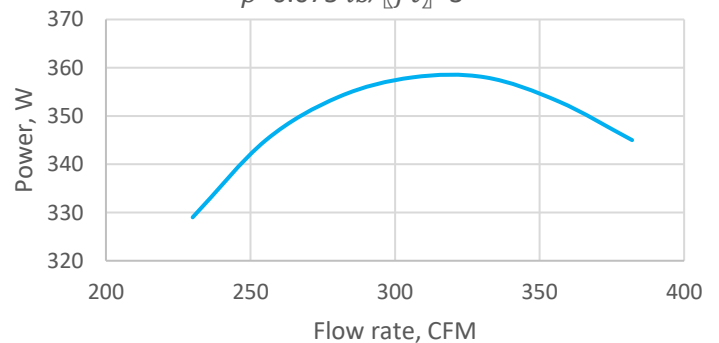
Force 110 Power Curve
