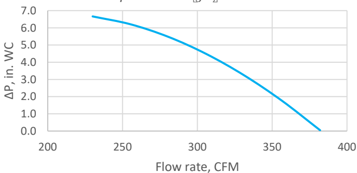
Force 110 Performance Curve
